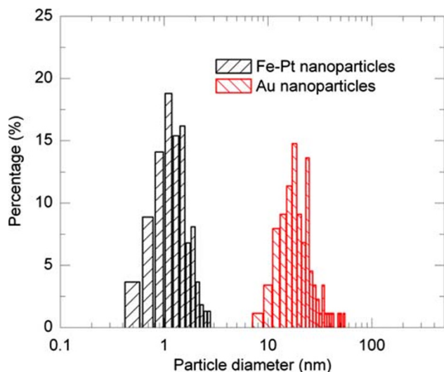
Fig. 11 Comparison of size distributions between Fe–Pt nanoparticles with a precursor of \text{Fe(II)Cp}_2/\text{Pt(II)(acac)}_2 = 4.0/6.0 mM (300 mJ, 50 Hz, 15 W) and Au nanoparticles with a laser pulse frequency of 2 Hz
