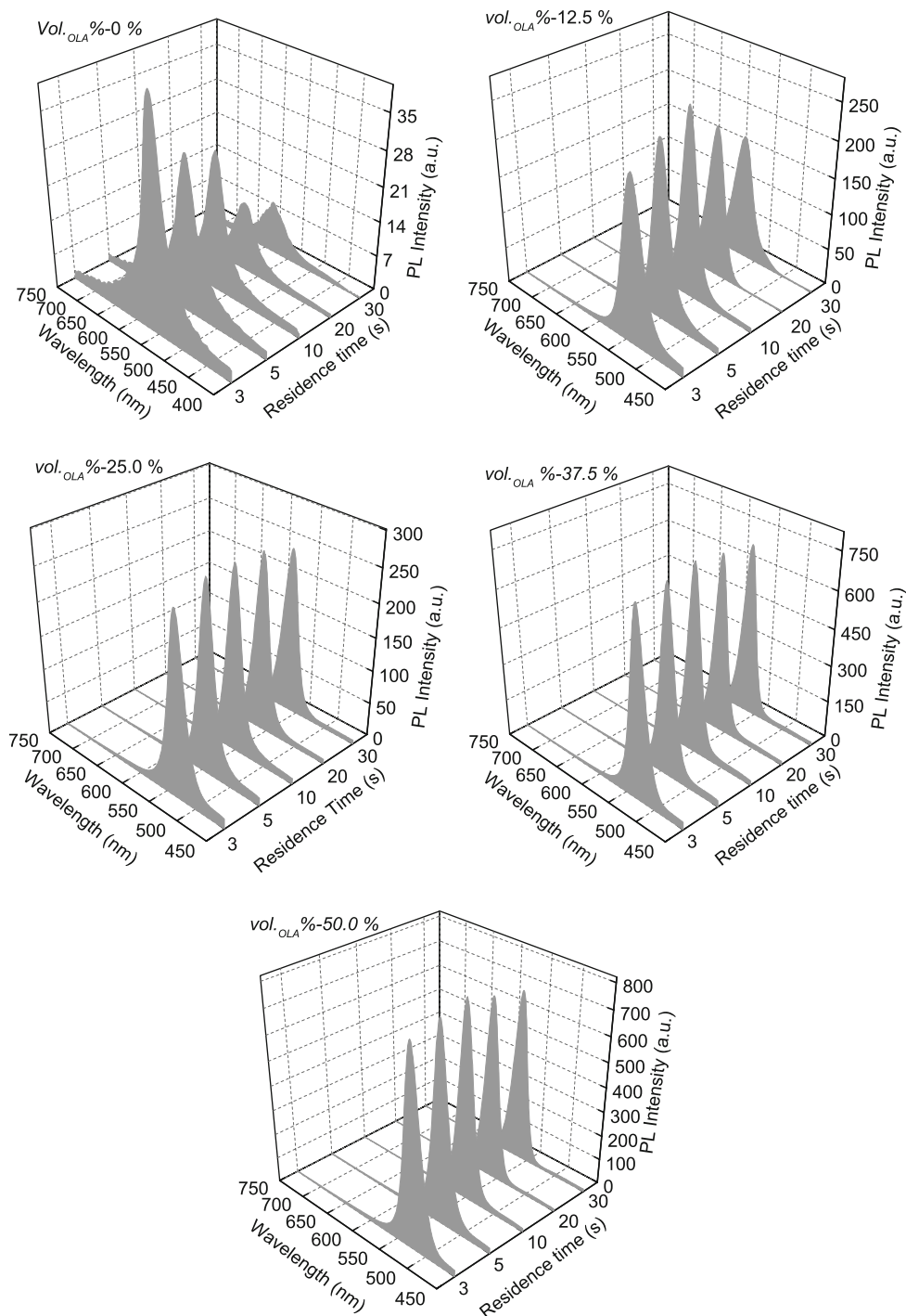
Fig. 6 PL spectra of the CdSe samples monitored during the evolution of residence time and volume percentage of OLA (OLA both in Cd and Se side, T = 280\text{ }^{\circ}\text{C} )
