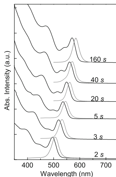
Fig. 8 A size series of CdSe NCs synthesized by the variation of residence time from 2 s to 160 s ( \text{vol.}_{\text{OLA}}\% = 3\text{ mL} , T = 280\text{ }^{\circ}\text{C} )
