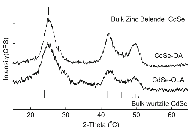
Fig. 10 XRD pattern of 3.6 nm CdSe NCs synthesized at 160 s ( \text{vol.}_{\text{OLA}}\% = 37.5\% , T = 280\text{ }^{\circ}\text{C} )
