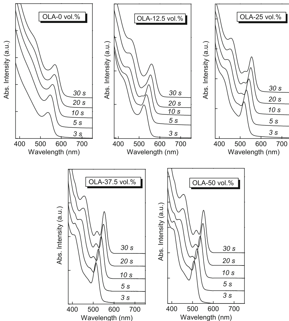
Fig. 4 Absorption spectra of the samples monitored during the evolution of residence time and the volume percentage of OLA (OLA both in Cd and Se side, T = 280\text{ }^{\circ}\text{C} )
