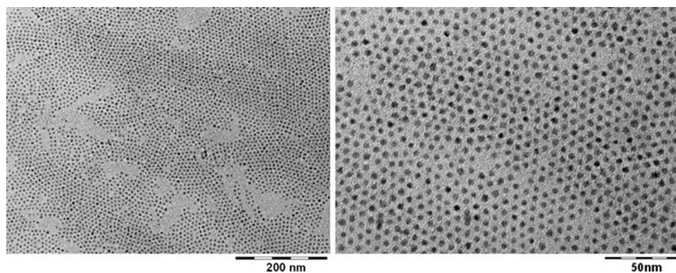
Fig. 9 TEM images of 3.6 nm CdSe NCs synthesized at 160 s ( \text{vol.}_{\text{OLA}}\% = 37.5\% , T = 280\text{ }^{\circ}\text{C} )
