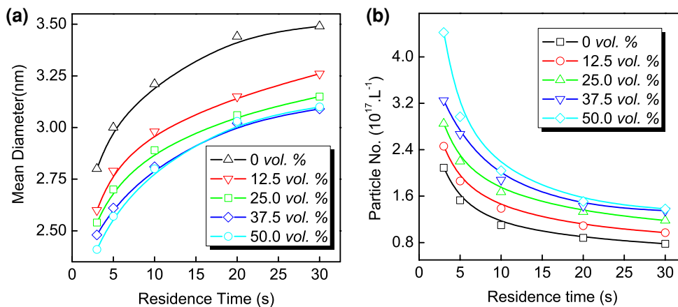
Fig. 5 a Mean diameter, b particle concentration of the CdSe samples obtained during the evolution of residence time and volume percentage of OLA (OLA both in Cd and Se sources, T = 280\text{ }^{\circ}\text{C} )
