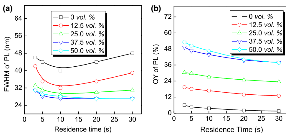
Fig. 7 a FWHM of PL and b QY of the CdSe samples obtained during the evolution of residence time and volume percentage of OLA (OLA both in Cd and Se sources, T = 280\text{ }^{\circ}\text{C} )
