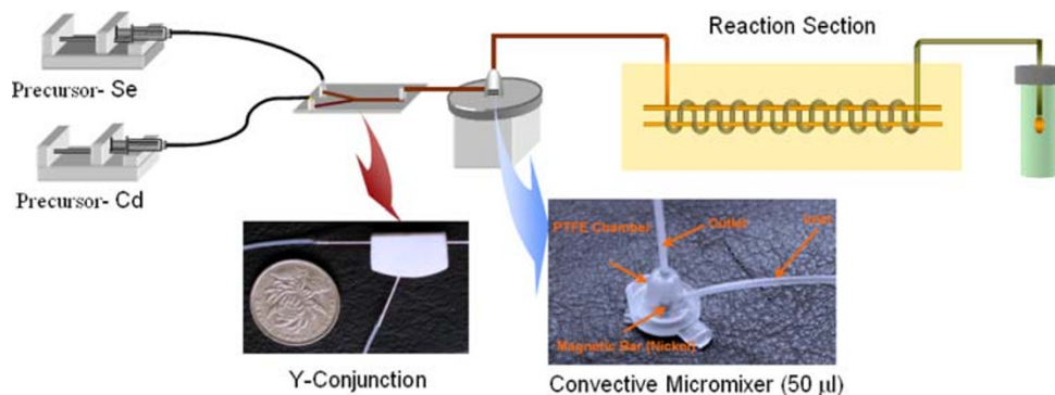
Fig. 1 Schematic graph of the microfluidic capillary reactor
