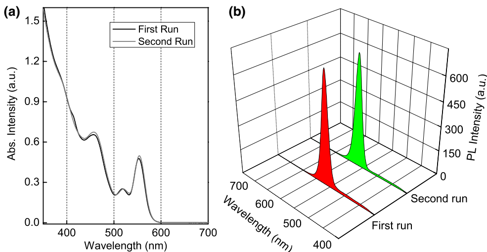
Fig. 2 a Absorption and b PL spectra of CdSe NCs prepared in two independent operations under the same reaction condition ( \text{vol.}_{\text{OLA}}\% = 37.5\% , T = 280 °C, t = 20 s)
