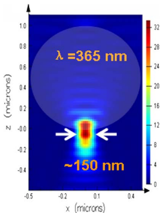
Fig. 1 One example of the focus process by the silica micro-sphere of 1 \mu\text{m}
