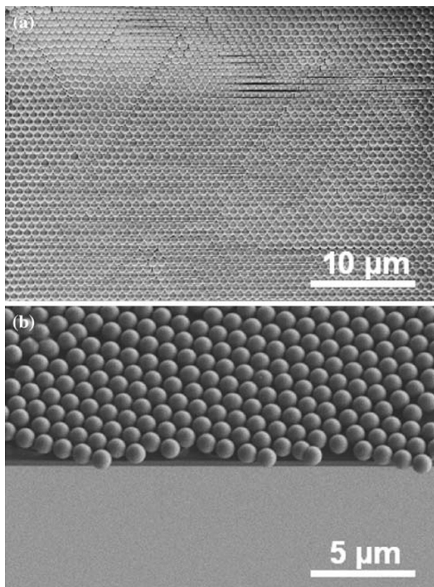
Fig. 5 (a) A typical SEM image of a large area of HCP monolayer of silica microspheres forming on top of photoresist; (b) the tilted view of the spheres on photoresist
