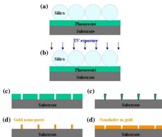
Fig. 3 The schematic process of NSP for fabrication nanostructures; from (b) to (c), it switches to two different processes with positive or negative photoresist used
