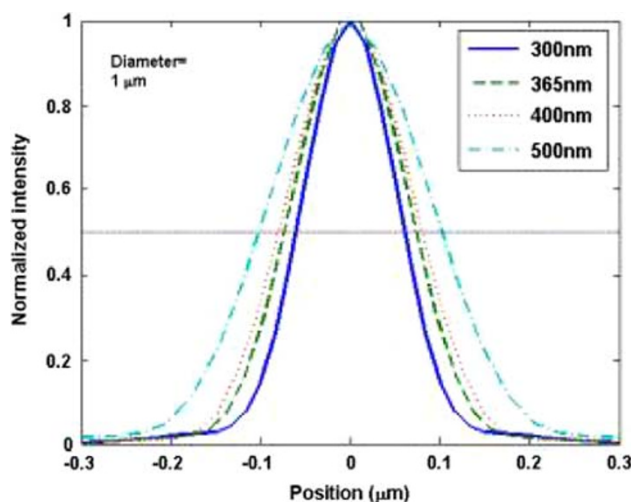
Fig. 2 The normalized intensity of the focused light versus the position with different wavelengths of UV light
