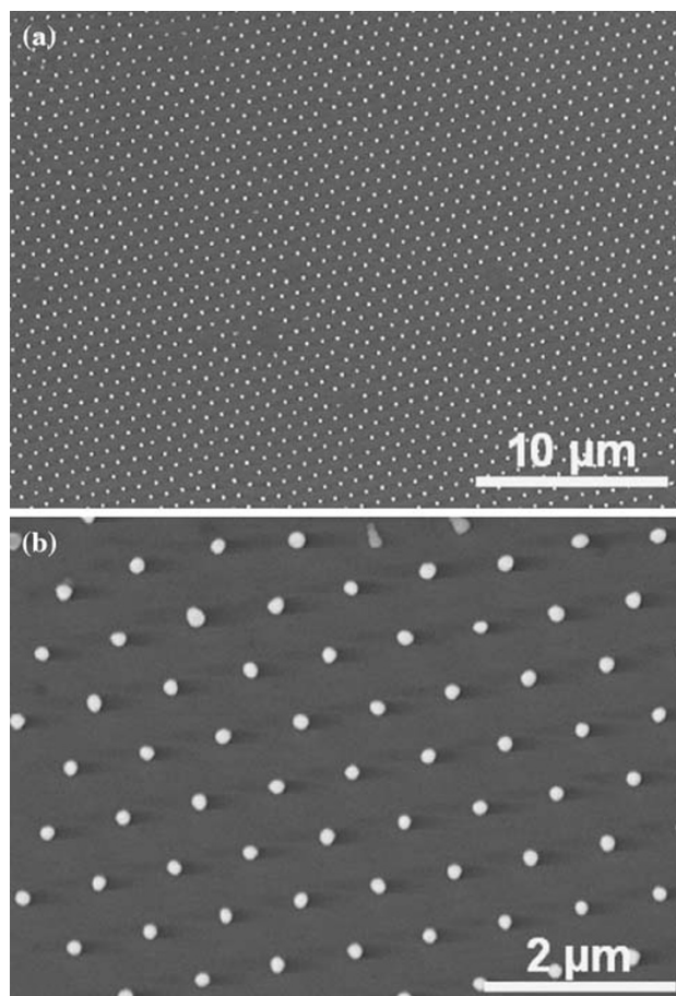
Fig. 6 (a) A typical SEM image of a large area of uniform nanopillars of photoresist after development; (b) the enlarged view of the nanopillars
