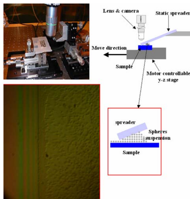
Fig. 4 The setup used for forming a large area of HCP micro-/nanospheres and one snap shot of the spheres forming HCP monolayer
