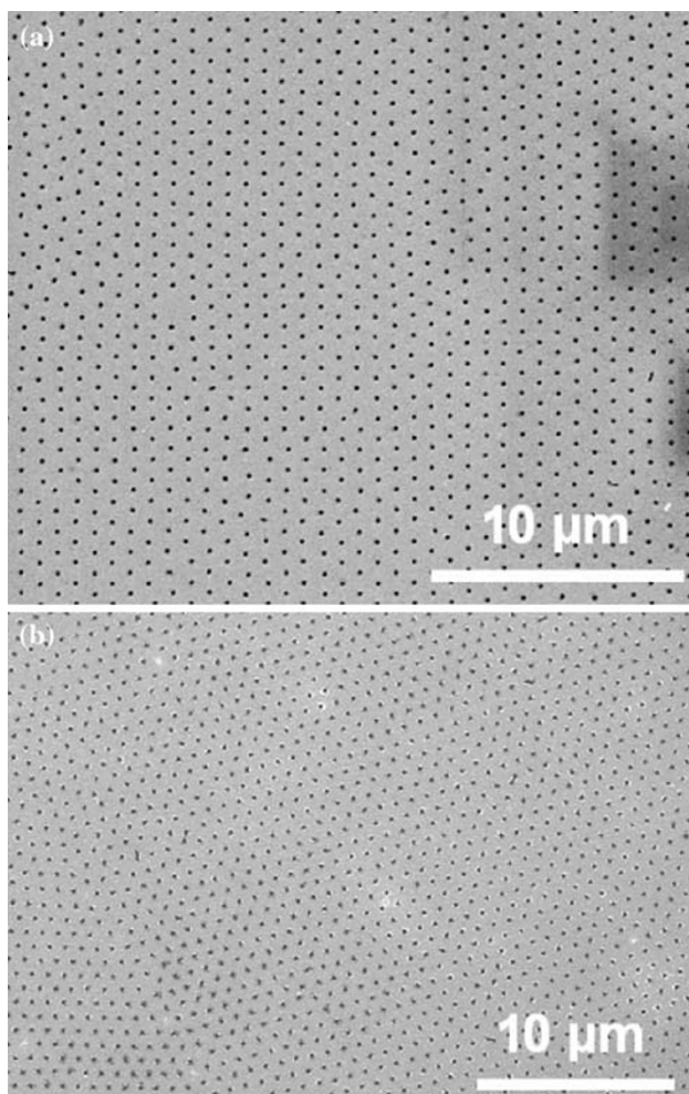
Fig. 7 SEM images of hexagonal distributed uniform nanoholes (diameter of about 180 nm) perforated in the gold (a) and aluminum (b) films fabricated by our lithography technique combined with lift-off process
