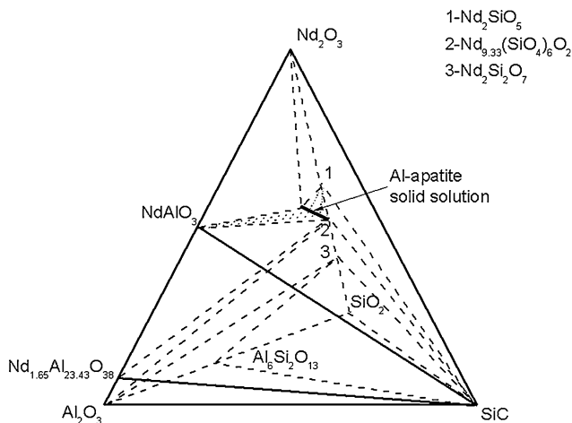
Fig. 10 Tentative phase diagram of the \text{SiC-Al}_2\text{O}_3\text{-Nd}_2\text{O}_3\text{-SiO}_2 (Si-Al-Nd-O-C) quaternary system at 1250 °C
