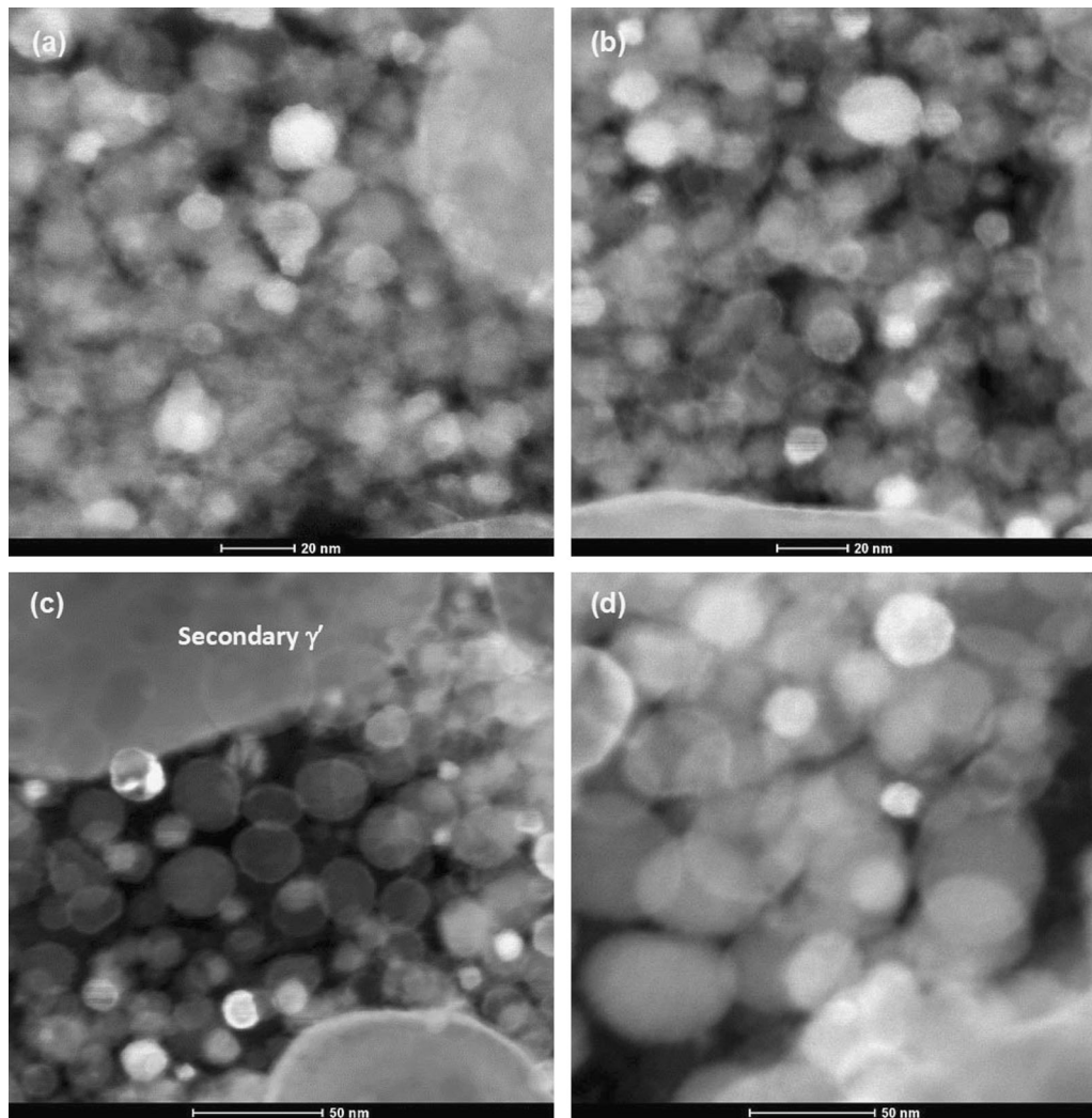
Fig. 2—Representative STEM dark-field micrographs showing tertiary \gamma' precipitates after different thermal exposure time at 700 °C: (a) as-received, (b) 50 h, (c) 100 h, and (d) 500 h. Note the different magnifications between (a) and (b) and (c) and (d).
