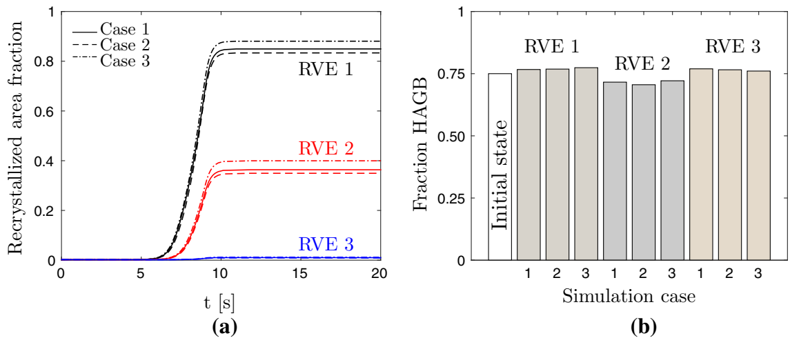
Fig. 15—(a) Recrystallized area fraction vs time for the different simulation scenarios. The line color indicates the RVE and the line type which case, cf. Table II. (b) Length-weighted fraction of high-angle grain boundaries (HAGB) at the end of the different annealing scenarios.
