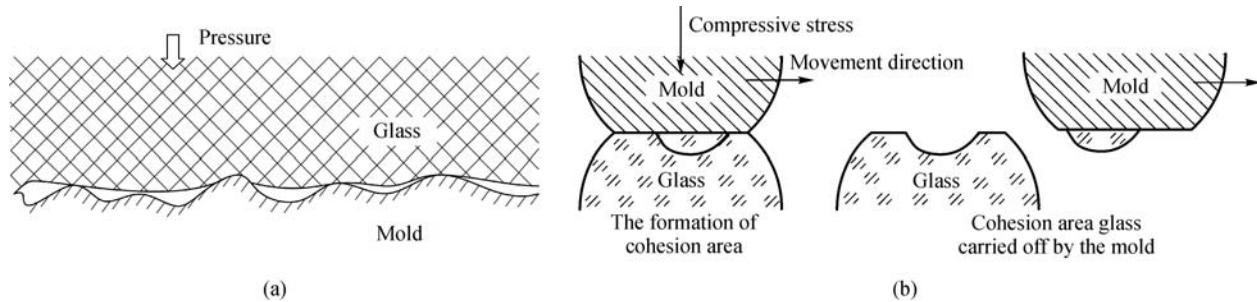
Fig. 34 Frictional contact model on the glass-mold interface. (a) Global view; (b) regional view
