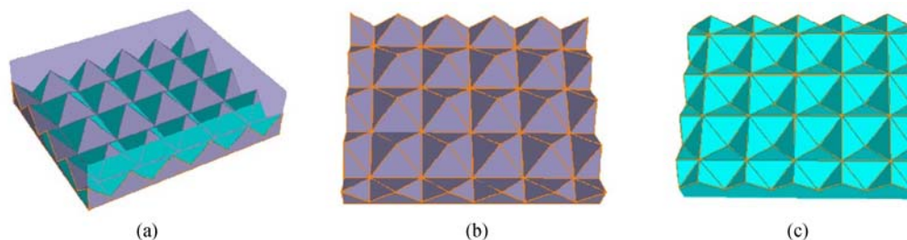
Fig. 5 Glass molding technology of microstructure array. (a) Forming schematic of the microstructure array; (b) mold with microstructures; (c) glass with microstructures [34]
