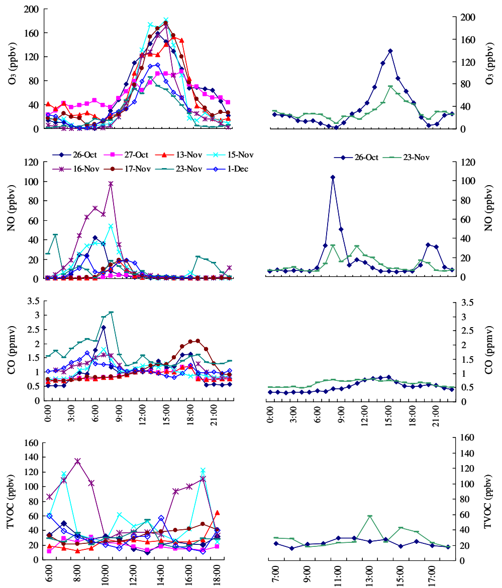
Fig. 4 Diurnal variations of O 3 , NO, CO, and TVOC on O 3 episode days at WQS and TC
