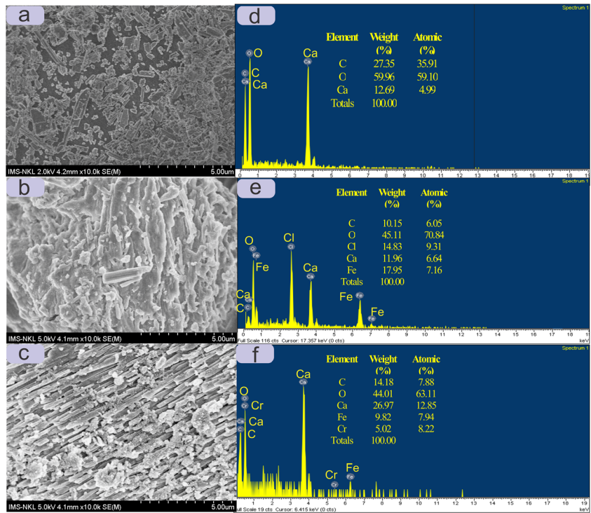
Fig. 1S. SEM and EDS of (a, d) snail shell (SS), (b, e) magnetic snail shell (MSS25), and (c, f) magnetic snail shell after Cr(VI) adsorption (MSS25–25) (replaced Fig. 2)
