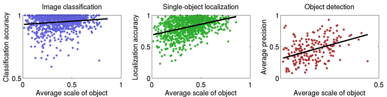
Fig. 13 Performance of the “optimistic” method as a function of object scale in the image, on each task. Each dot corresponds to one object class. Average scale ( x-axis ) is computed as the average fraction of the image area occupied by an instance of that object class on the ILSVRC2014 validation set. “Optimistic” performance ( y-axis ) corresponds to the best performance on the test set of any entry submitted
