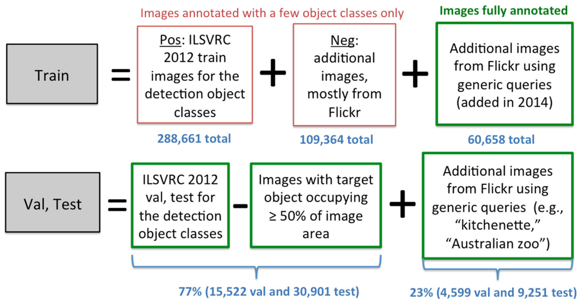
Fig. 3 Summary of images collected for the detection task. Images in green (bold) boxes have all instances of all 200 detection object classes fully annotated. Table 5 lists the complete statistics
