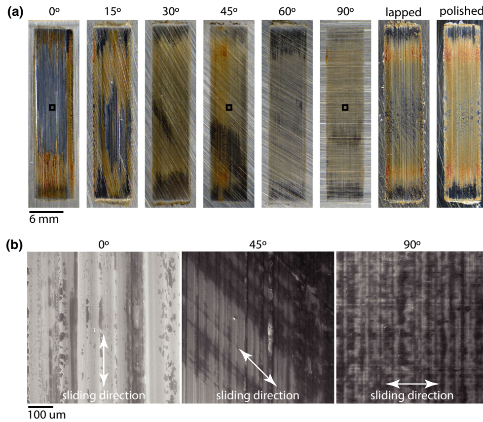
Fig. 4 Transfer films. a Optical images of transfer films for each countersample. b Scanning electron micrographs of the 0°, 45° and 90° wear tracks. The transfer films are visibly more continuous and uniform as the roughness angle approaches 90°
