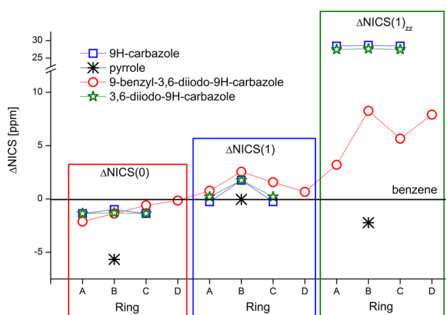
Fig. 5 B3LYP/6-311++G(3df,2pd) calculated differences ( \Delta NICS) in aromatic indices for different rings of pyrrole, 9H-carbazole and 9-benzyl-3,6-diiodo-9H-carbazole and 3,6-diiodo-9H-carbazole (benzene was used as reference model for the \Delta NICS indices)
