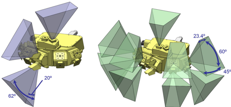
Fig. 5 The field-of-view of the three ion eyes are shown on the left . The two more equatorial eyes are cocked to avoid scanning the ecliptic plane to keep the Sun out of the field of view. The field-of-view of the nine electron eyes are shown on the right . The trapezoidal shape resulted from the efforts to minimize the blockage resulting from spacecraft appendages with little loss of solid-angle coverage. In the left hand panel it can be seen that there is 180^\circ angular coverage
