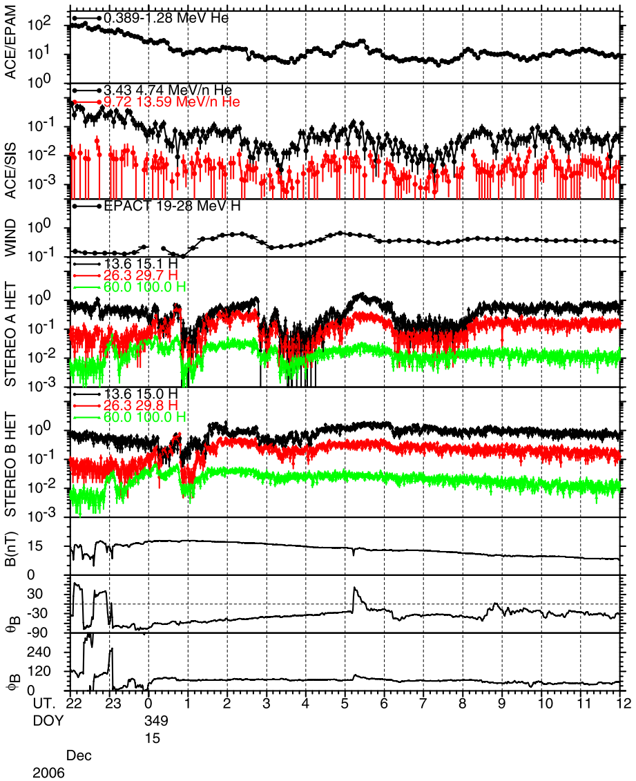
Figure 4 Energetic particle observations from Wind , ACE and STEREO illustrating that the intensity variations at STEREO were also observed around 20 minutes earlier at Wind and ACE, in orbit around L_1 (intensities are in units of (\text{MeV/n s cm}^2 \text{sr})^{-1} ). The bottom panels show the magnetic field intensity and polar and azimuthal angles at STEREO A in GSE coordinates.
