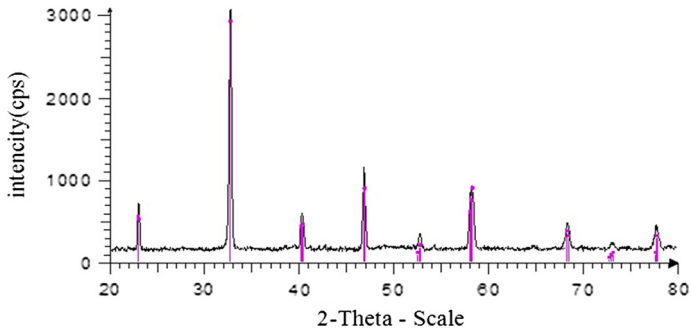
Fig. 7 XRD pattern of the GSFO NPs calcined at 700 °C
