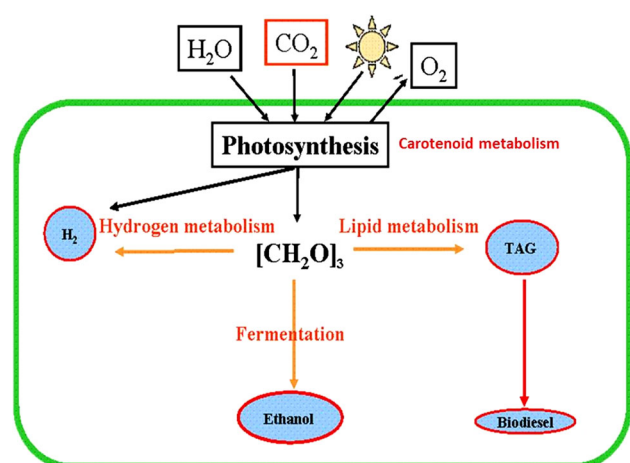
Fig. 1 Metabolic pathways linked to biofuel production in green algae
