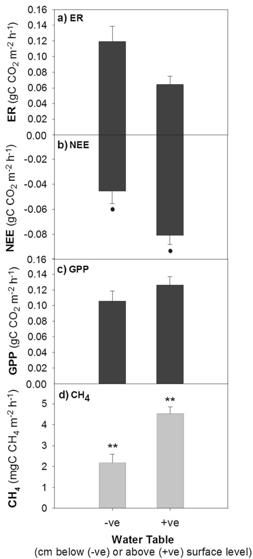
Fig. 3 Average a) Ecosystem Respiration b) Net Ecosystem Exchange and c) Gross Primary Production fluxes ( \text{g C CO}_2 \text{ m}^{-2} \text{ h}^{-1} ) and d) \text{CH}_4 flux ( \text{mg C CH}_4 \text{ m}^{-2} \text{ h}^{-1} ) at sample locations in Barrow (BES, BEO and BEN) and Ivotuk split by sites where water table height is below (-ve) or above (+ve) surface level (cm). Bars represent means with error bars shown as standard errors. ** denotes bars are significantly different at p < 0.01 , • denotes p < 0.1
