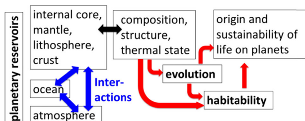
Fig. 1 Sketch on the themes involved in Planet TOPERS. Note that this sketch is done for all terrestrial planets including the Earth
