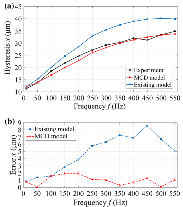
Fig. 17 Accuracy verification of the MCD model in hysteresis calculations
