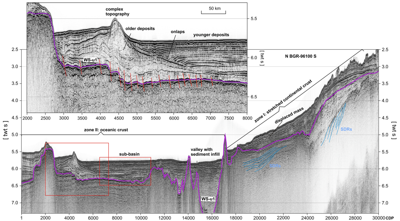
Fig. 5 Multichannel seismic line from the continental slope to the eastern flank of Maud Rise in the Lazarev Sea. The long seismic profile demonstrates sedimentation processes from continental slope
