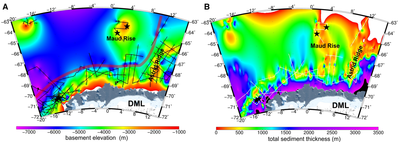
Fig. 9 a Depth to acoustic basement. The thick, dark red curve is a proposed Weddell Gyre pathway between Antarctica and Maud Rise. b Total sediment thickness at the Lazarev Sea and DML margin. The
