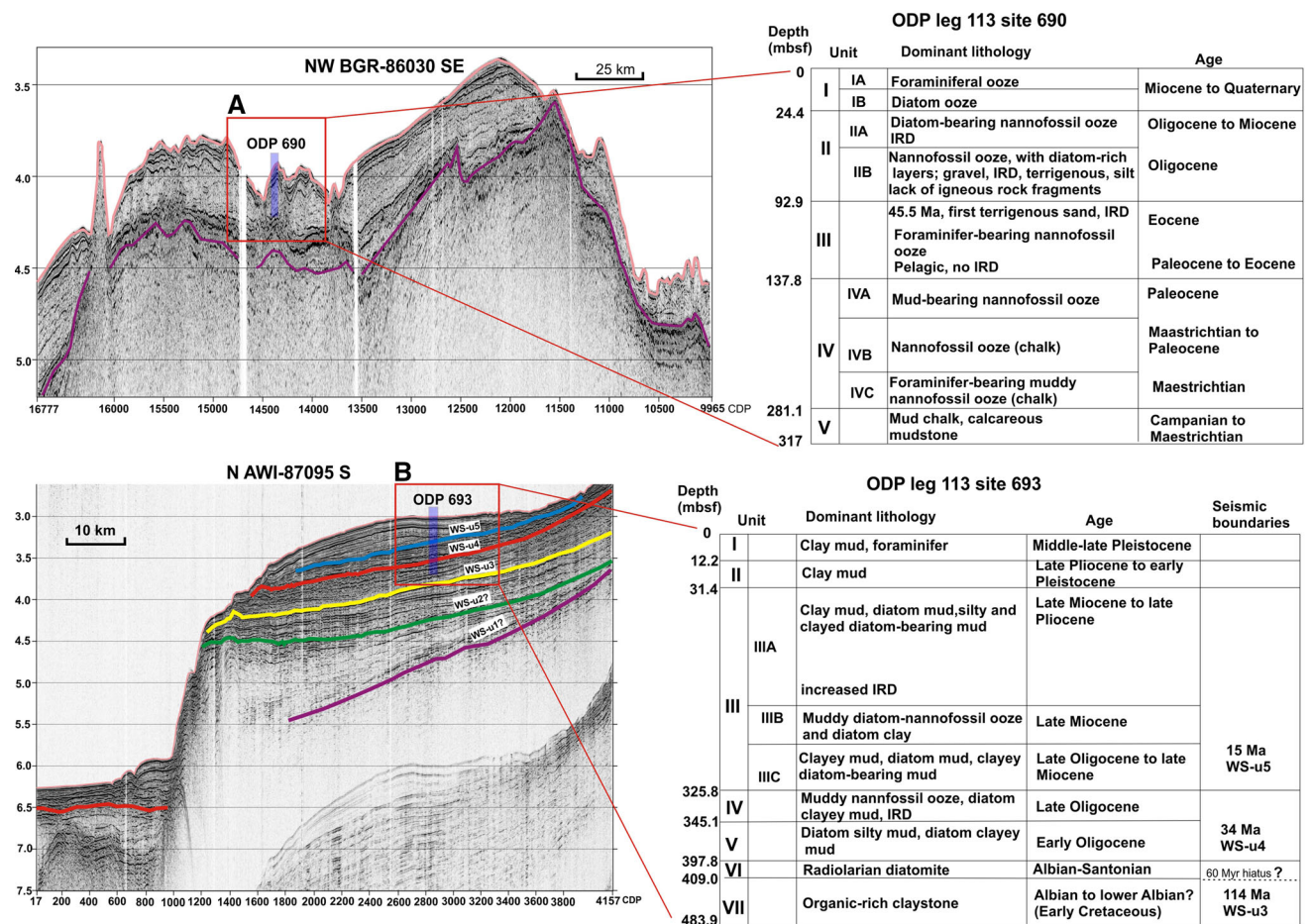
Fig. 2 The locations of ODP 690, 693 on the multichannel seismic lines from DML margin A and Maud Rise B. The tables at the right show the recovered dominant lithologies and accompanying age information from the two ODP samples, see Fig. 1 for location
