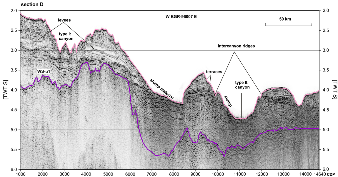
Fig. 8 Two types of canyons with different dimensions and formation mechanisms are distinguished on the multichannel seismic line, west of Astrid Ridge, see Fig. 1 for location
