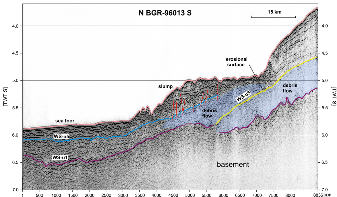
Fig. 4 Interpreted large-scale debris flow deposits and slumps in multichannel seismic data. Red lines signify interpreted growth faults, see Fig. 1 for location
