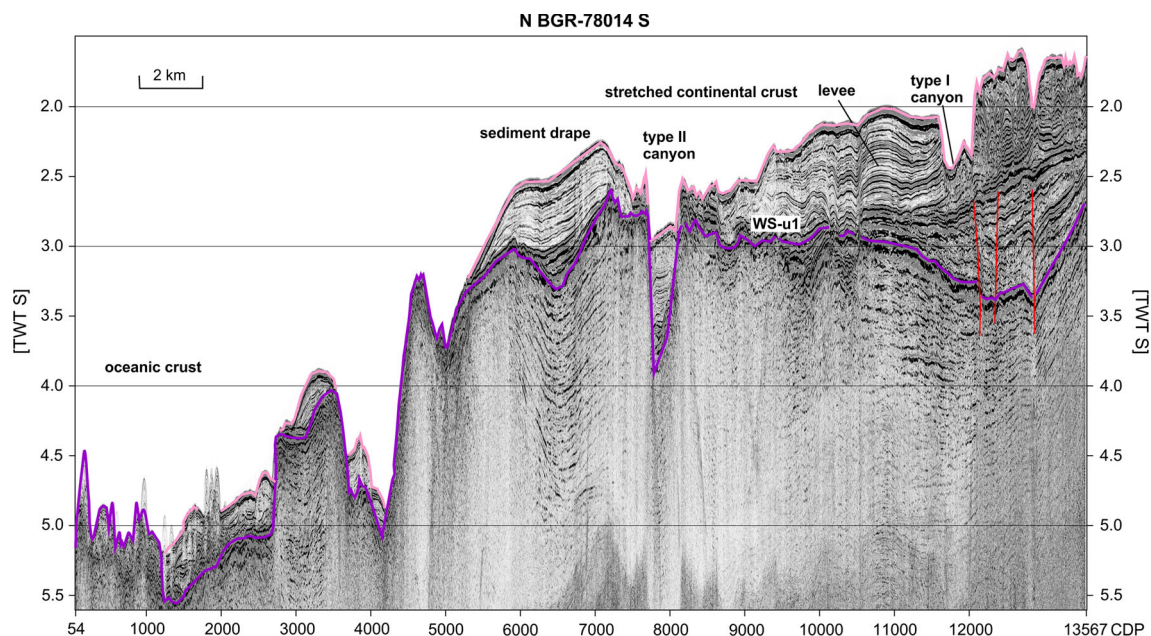
Fig. 7 The interpreted multichannel seismic line BGR-78014 crosses the Astrid Ridge. The line crossed both continental crust (CDP: 4500–13,567) and oceanic crust (CDP: 54–4500), which are situated
