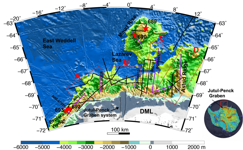
Fig. 1 Location of study area and available datasets. The background map depicts topography and bathymetry. The black lines represent multichannel seismic lines in the study region. The purple lines in section A, B, C and D are profiles presented in the study. The red stars represent the ODP drilling sites
