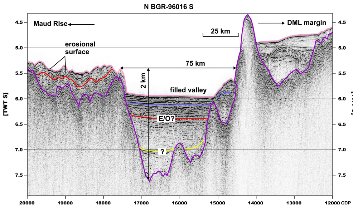
Fig. 6 A filled valley separating Maud Rise from Antarctica. Three unconformities are recognized in the fill sediment strata, see Fig. 1 for location
