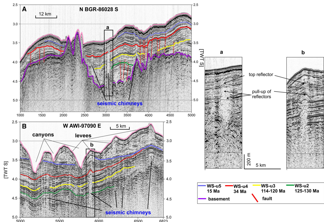
Fig. 3 Examples of pipe-like features, characterized by reflection-poor columns. The pipe-like features are interpreted as seismic chimneys in this study
