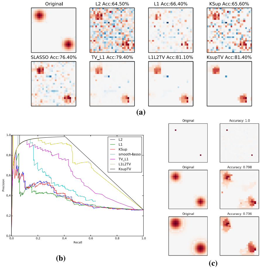
Fig. 3 a (left top to bottom right) ideal weight vector, weight vector obtained with \ell_1 , \ell_2 , k -support norm, TV + \ell_1 , and k -support/TV regularizer, and weight vector with combined total variation and k -support norm regularizer. The k -support/TV regularization gives the highest accuracy, support recovery, stability, and most closely approximates the target pattern. b Illustrates the improved precision-recall for k -support/TV versus the other methods on the support recovery for different thresholds. c Recovered support for varying ideal weight vector. This demonstrates that the k -support/TV regularization works well for a wide range of sparsity, correlation, and smoothness
