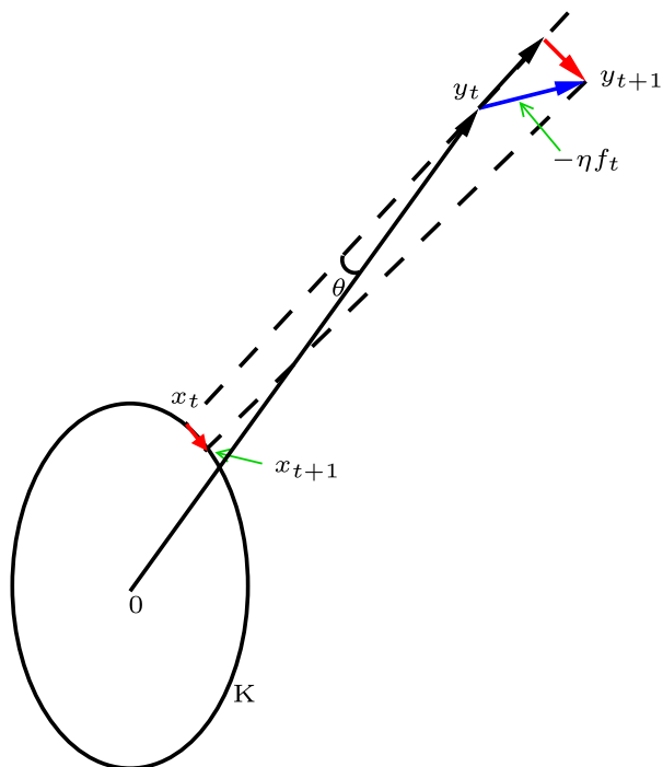
Fig. 1 The distance between successive projections, viz. \|x_t - x_{t+1}\| , is bounded by the length of the component of -\eta f_t orthogonal to the y_t - x_t
