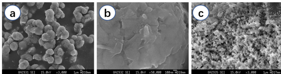
Fig. 4 Micrographs of ABGM1 (a, b) at different magnification and ABGM3 (c)
