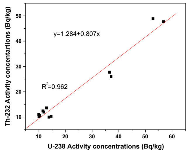
Fig. 4 Correlation between ^{232}\text{Th} and ^{238}\text{U} activity concentrations in the sand samples from Zonguldak beaches
