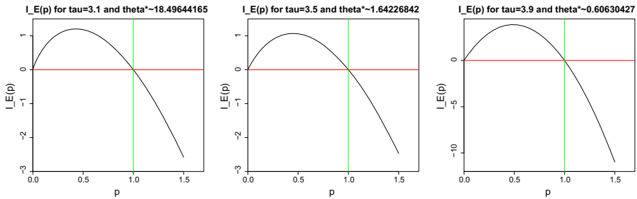
Fig. 1 Numerical plots of p \mapsto I_E(p) for \tau = 3.1, 3.5 and 3.9 . In a first step, \theta^* was determined as the unique \theta such that I_E(1) = I_E(1, \theta) = 0
