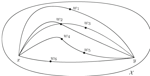
Fig. 3 Illustration of the notion of gate between two configurations x and y . The case depicted here is the following: \mathcal{S}(x, y) = \{w_1, \dots, w_6\} . The optimal paths in \Omega_{x,y}^{\text{opt}} are represented by the five black lines. The minimal gates are \{w_1, w_2, w_4, w_6\} and \{w_1, w_2, w_5, w_6\} . Any other subset of \mathcal{S}(x, y) obtained by adding some of the missing saddles to one of the two minimal gates is a gate
