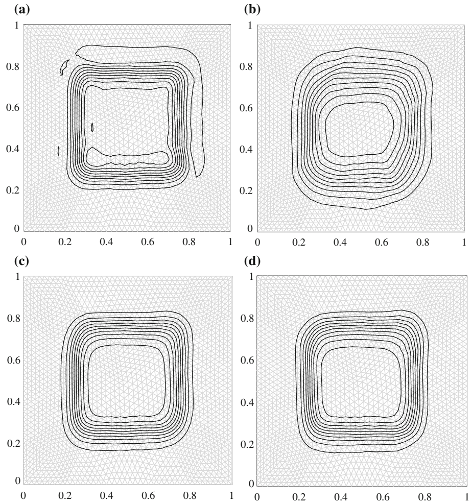
Fig. 8 Contours of the square wave at t = 1 with 3968 cells. a Unlimited. b SSL. c RSL. d ILR
