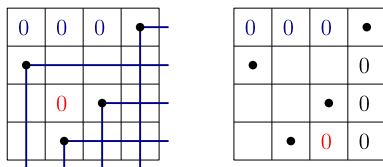
Fig. 9 Example of Proposition 6.10. For the permutation w = 4132 , the Rothe diagram is R_w = \{(1, 1), (1, 2), (1, 3), (3, 2)\} and the left-hull \overline{H_L(w)} = \{(1, 1), (1, 2), (1, 3), (2, 4), (3, 4), (4, 3), (4, 4)\} . The map \varphi is given by (1, j) \mapsto (1, j) for j = 1, 2, 3 and (3, 2) \mapsto (4, 3)
