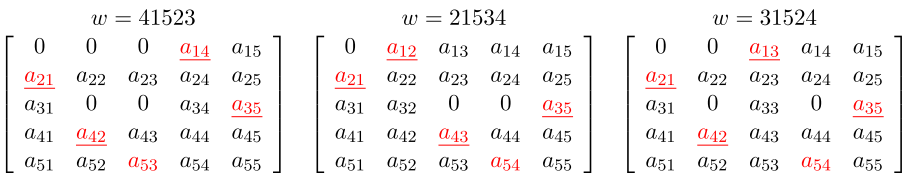
Fig. 5 Representative matrices counted by \text{mat}_q(5, R_w, r) where R_w is a Rothe diagram and w is (i) 41523 (vexillary), (ii) 21534 (skew-vexillary), (iii) w = 31524 (not skew-vexillary). The entries a_i w_i are in red
