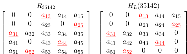
Fig. 7 Matrices indicating the (i) Rothe diagram and (ii) left hull of w = 35142 . The matrix entries a_i w_i are in red
