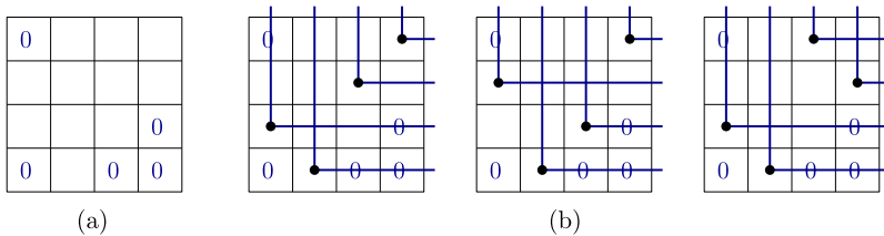
Fig. 4 (a) Set B with the NE Property. (b) Example of computing \text{mat}_q(n, \overline{B}, r) when B has the NE Property. There are three placements of four rooks in B with 0, 1, and 1 NE-inversions, respectively. By Theorem 4.2, \text{mat}_q(4, \overline{B}, 4) = (q - 1)^4 q^{11-4} (1 + 2q^{-1})
