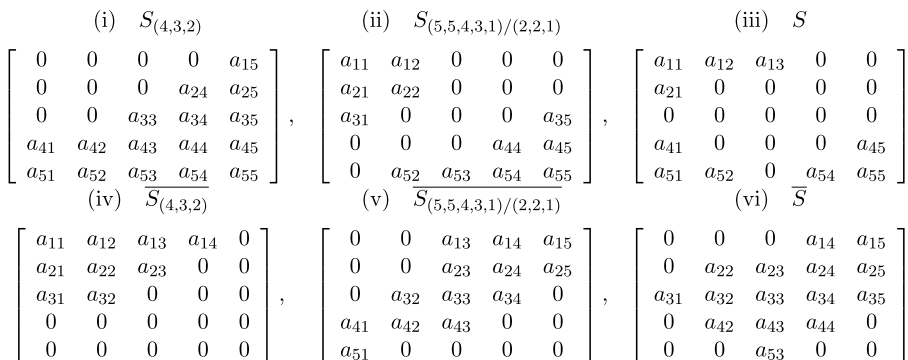
Fig. 2 Representative matrices from \text{mat}_q(5, S, r) when S is (i) a straight shape, (ii) a skew shape, (iii) a set with the NE Property; and their respective complements (iv), (v), (vi)
