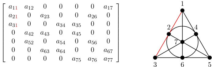
Fig. 1 A representative matrix counted in \text{mat}_q(7, F, 7) where F is the complement of the point-line incidence matrix of the Fano plane, shown at right. Stembridge [18] showed this to be the smallest example of the form \text{mat}_q(n, S, n) that is not a polynomial in q
