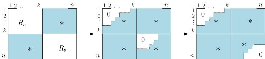
Fig. 6 If w can be decomposed as a_1 a_2 \cdots a_k b_1 b_2 \cdots b_{n-k} where a_i < b_j and both a = a_1 a_2 \cdots a_k and b = b_1 b_2 \cdots b_{n-k} are 2143 avoiding, then \overline{R_w} can be rearranged into a skew shape
