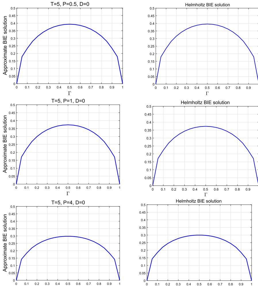
Fig. 12 \varphi(x, T) on \Gamma , for D = 0 and different values of P (left), together with the corresponding Helmholtz BIE static approximate solution (right), having fixed \theta = \pi/3
