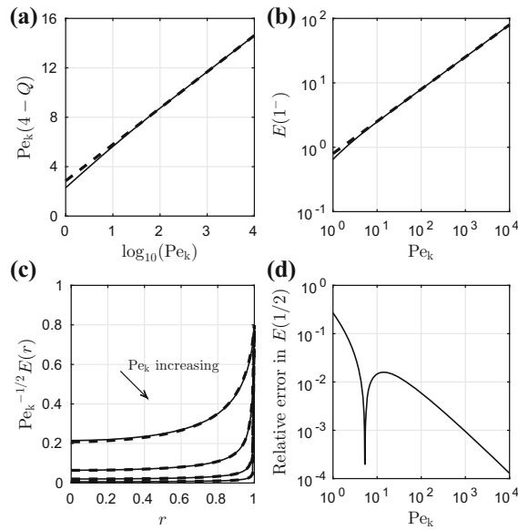
Fig. 3 Validation of the leading-order asymptotic results (89), (91), and (92) against the finite- Pe_k solutions. In a , we plot Pe_k(4 - Q) as a function of \log_{10}(Pe_k) . The solid curve is the finite- Pe_k solution (36), while the dashed line is a linear fit for large values of Pe_k (between 10^2 and 10^4 ). In b , we plot the evaporation rate at the contact line E(1^-) as a function of Pe_k . The solid curve is the finite- Pe_k solution (33), while the dashed line is the large- Pe_k asymptote (91). c Scaled evaporation rate Pe_k^{-1/2}E(r) as a function of r for Pe_k = 10^1, 10^2, 10^3, 10^4 . The solid curves are the finite- Pe_k solution (32) and the dashed curves show the leading-order asymptotic prediction (95). d The relative error in E(1/2) between the finite- Pe_k solution (32) and the leading-order asymptotic prediction (95).
