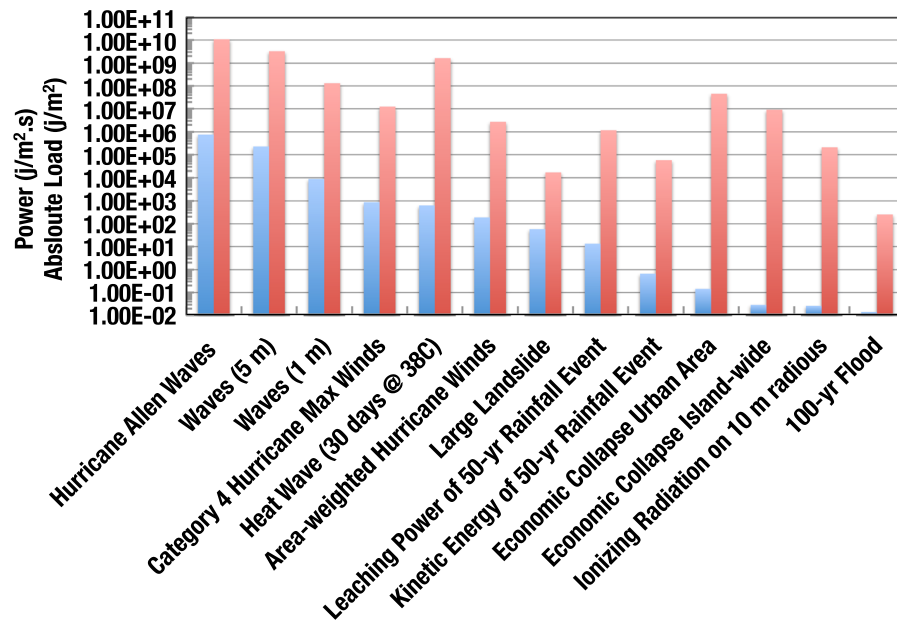
Fig. 10 Power (first bars) and absolute load (second bars) of extreme events or their component disturbance forces. These estimates are based on real values observed in Puerto Rico over the last 100 years
