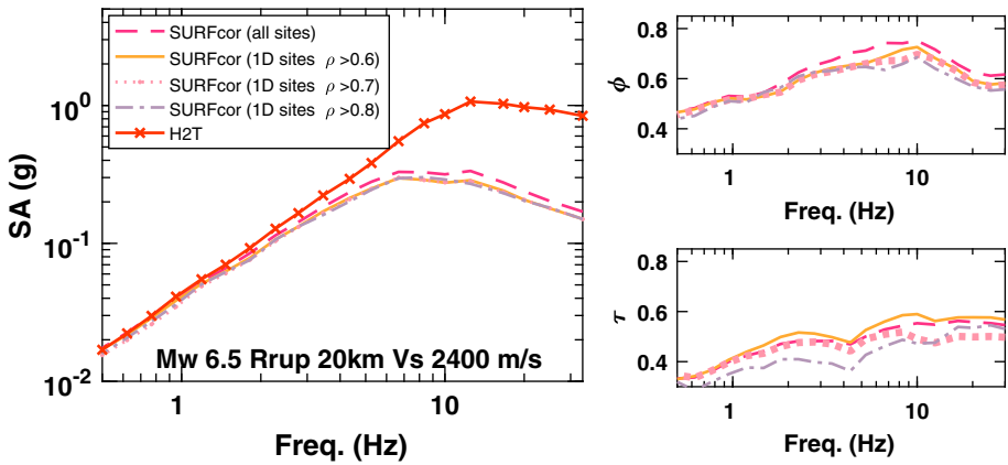
Fig. 12 Effect of the “1D” selection of sites on predicted SA for SURFcor ( left ) for a specific scenario ( M_W = 6.5 , R_{RUP} = 20 km) on a hard-rock site ( V_S = 2400 m/s), and on the within-event \phi ( right top ) and between-event \tau ( right bottom ) variability
