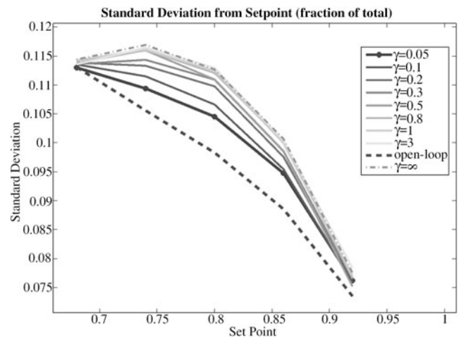
Fig. 11 Standard deviation of output for different setpoints and integrator constants \gamma . The dashed line at the bottom corresponds the standard deviation when the system is under open loop control. The dash-dot line at the top corresponds to the standard deviation of the system when driven with a bang-bang controller and the input is always saturated. Each standard deviation is estimated from 200 simulation trajectories
