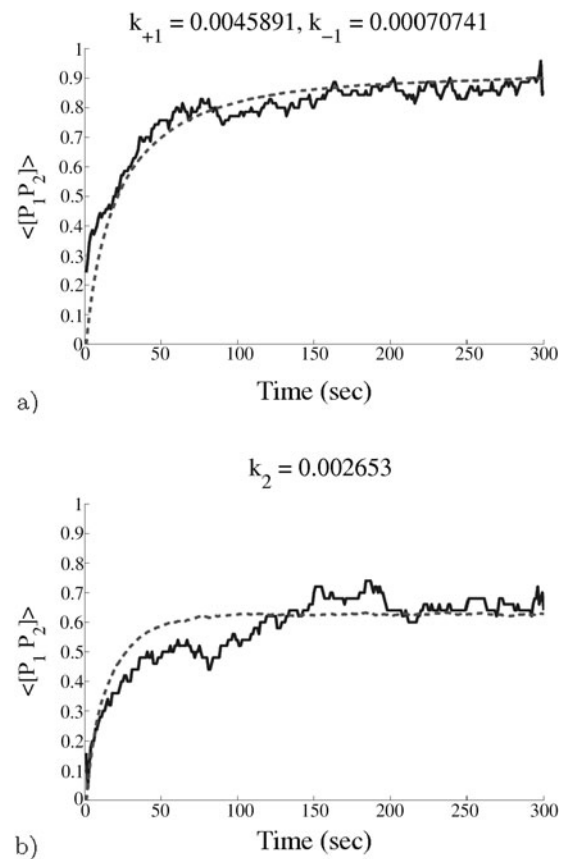
Fig. 5 Curve fitting results used to determine rate constants
