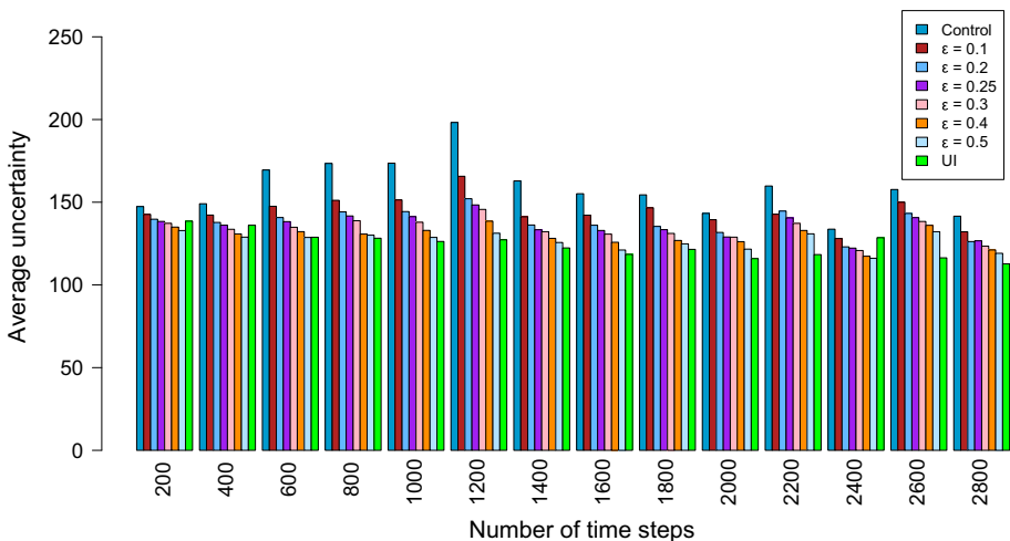
Fig. 13 Average uncertainty per 200 time steps across subjects during the training process for different \epsilon values and original Control and UI conditions. Note that from left to right, each bar represents the corresponding value for the original Control condition, \epsilon = 0.1 , \epsilon = 0.2 , \epsilon = 0.25 , \epsilon = 0.3 , \epsilon = 0.4 , \epsilon = 0.5 and the original UI condition, respectively (Color figure online)
