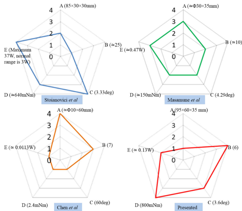
FIGURE 8. Comparison among five evaluation standards. Notes that rank 4 denotes the best in its corresponding standard. The larger the size of pentagon, the better is the overall performance in terms of A: motor dimension, B: number of components, C: step size, D: motor output torque, E: power.
