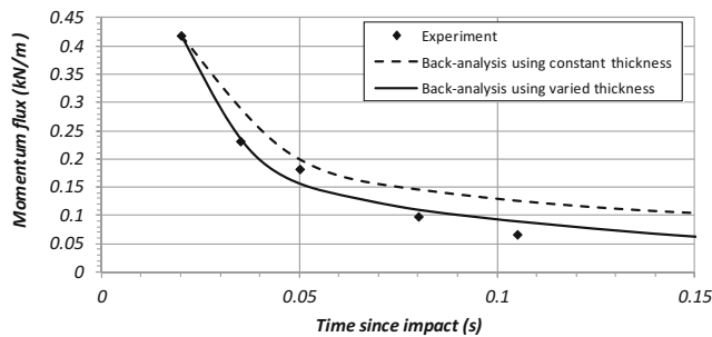
Fig. 13 Comparison of experimental and back-analysed momentum fluxes.
