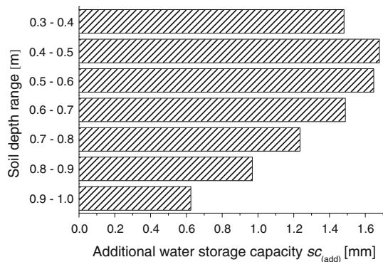
Fig. 12 Predicted additional water storage capacity sc_{(add)} according to Eq. (13) for different soil depth ranges at site A
