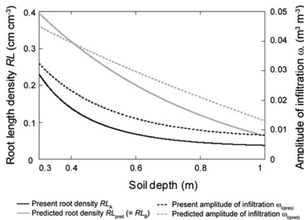
Fig. 11 Present ( RL_A ) and predicted root density ( RL_{pred} = RL_B ) according to Eqs. (8) and (9), and present and predicted amplitudes of infiltration \omega_{I(pres)} and \omega_{I(pred)} according to Eqs. (10) and (11) for site A
