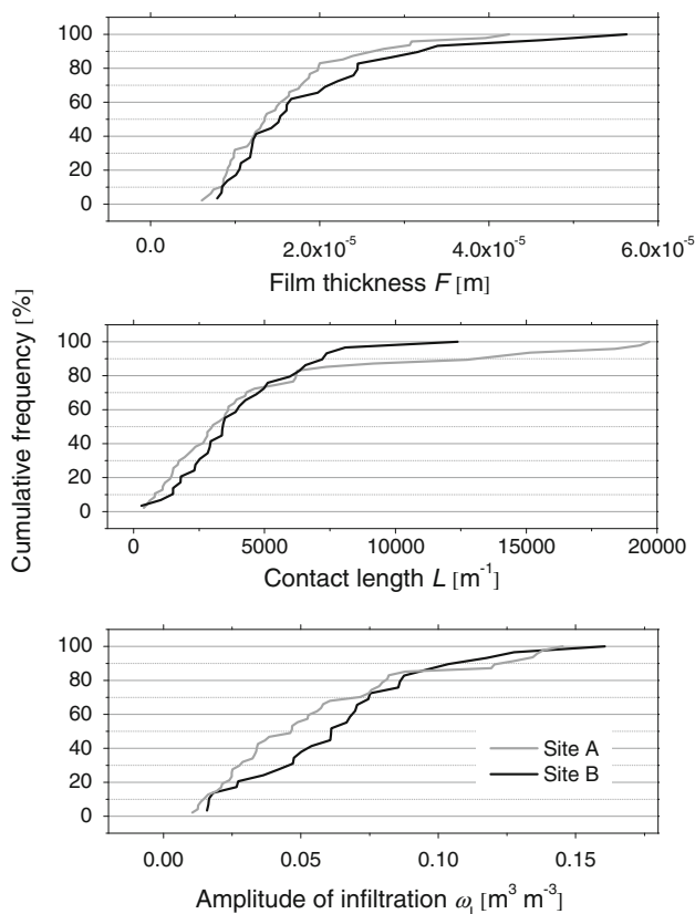
Fig. 8 Cumulative frequencies of contact lengths L , film thicknesses F and amplitudes of infiltration \omega_1 for the third irrigation at sites A ( n = 47 ) and B ( n = 29 ). Only water-content waves with \omega_1 \geq 0.01 \text{ m}^3 \text{ m}^{-3} were considered
