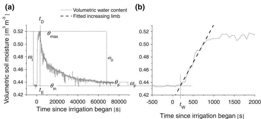
Fig. 5 a Definitions of parameters and variables of water-content waves ( wcw ). b Fitted increasing limb of a wcw . \theta_{in} initial volumetric water content, \theta_{max} maximum volumetric water content, \theta_F volumetric water content 75,000 s after the irrigation began, \omega_I \theta_{max} - \theta_{in} ,
