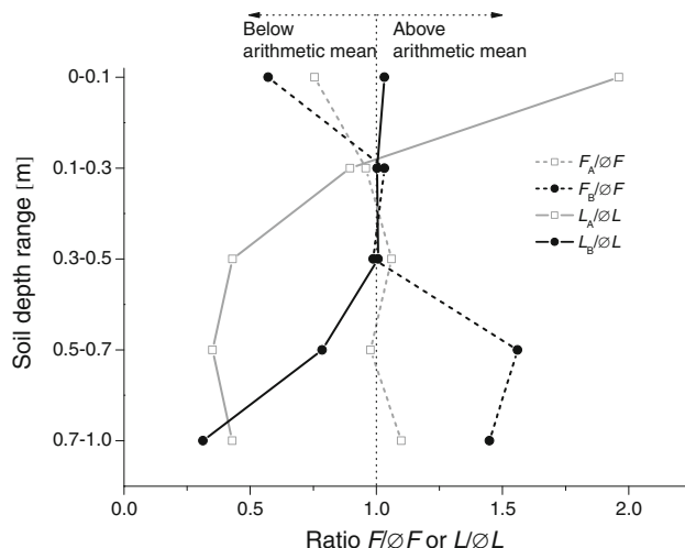
Fig. 9 Relative film thicknesses and contact lengths for sites A and B versus soil depth. F_A, F_B, L_A, L_B arithmetic means of the film thicknesses F and contact lengths L of the specific soil depth range at sites A ( F_A, L_A ) and B ( F_B, L_B ), \bar{F} and \bar{L} arithmetic means of the film thicknesses and contact lengths at the specific soil depth range, including both sites A and B
