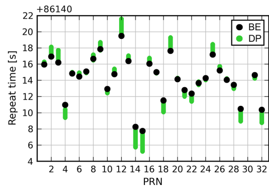
Fig. 5 Orbit repeat times calculated using elements in the broadcast ephemeris (BE) and the ranges of repeat times calculated by the dot product (DP) method for each GPS satellite PRN tracked at UCL on September 3, 2013
