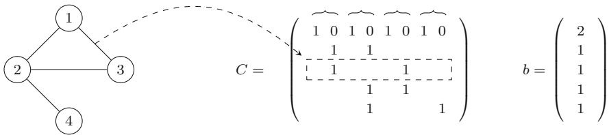
Fig. 5 Reduction from independent set to a column selection problem; here k = 2
