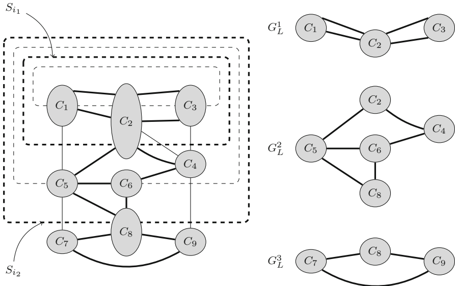
Fig. 2 An example showing G_L on the left (with the edges of G_L^A in bold), and the resulting G_L^j = (\mathcal{B}^j, A_L^j) for j \in \{1, 2, 3\}
