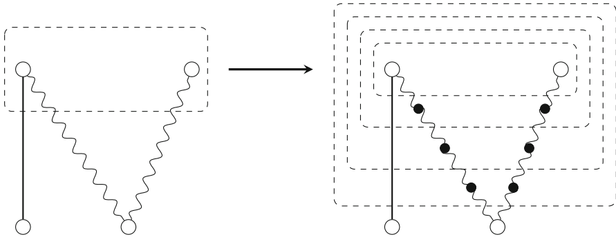
Fig. 4 Edge splitting ensures that there is no advantage to not taking all edges in E''
