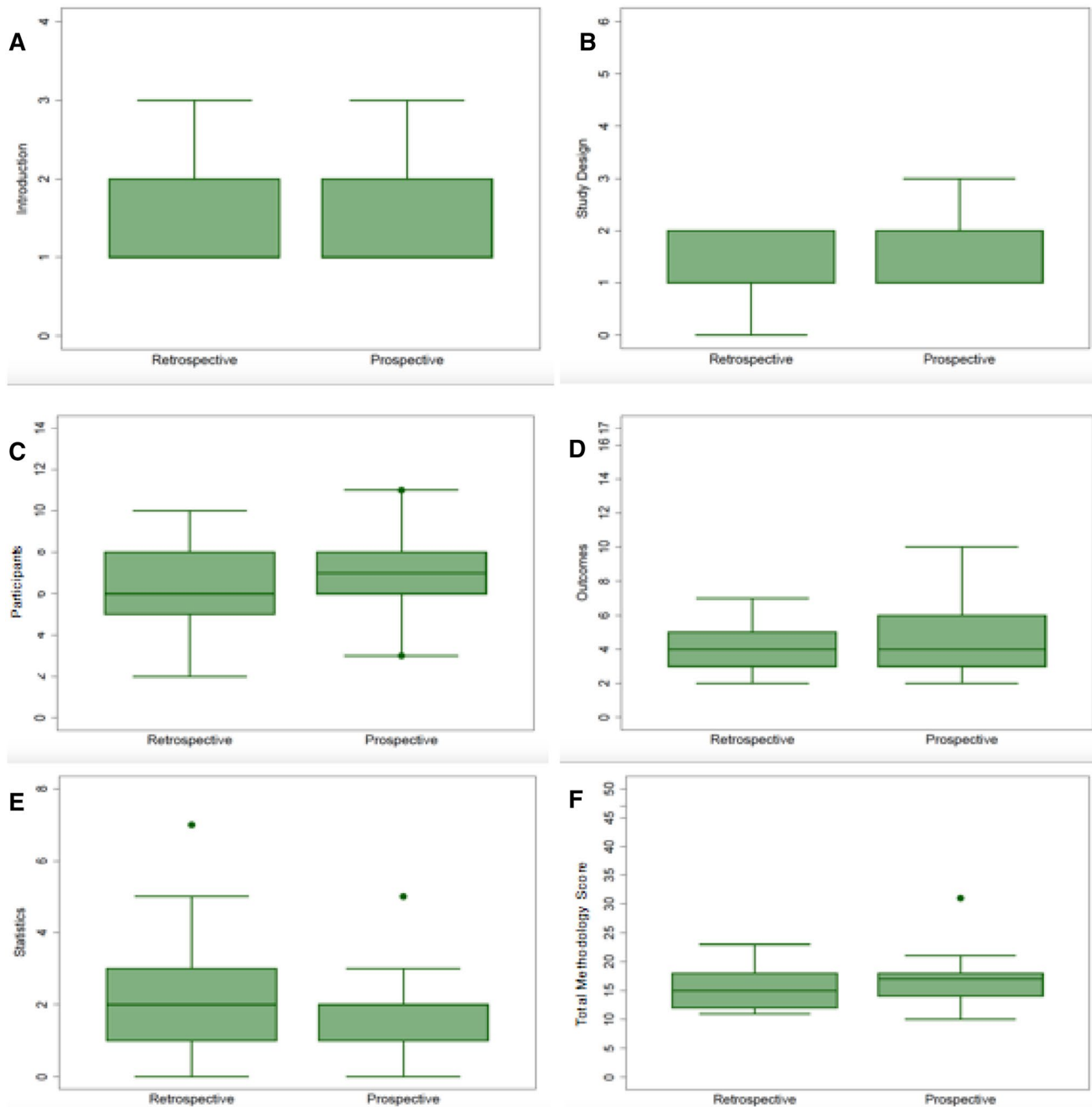
Fig. 3 Box and whisker plots showing methodology scores for prospective and retrospective studies. a Introduction, b study design score, c participants score, d outcomes score, e statistics score, f total methodology score
