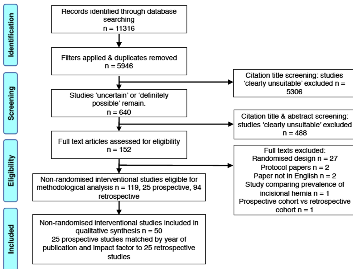
Fig. 1 PRISMA diagram showing selection of non-randomised interventional studies for this review
