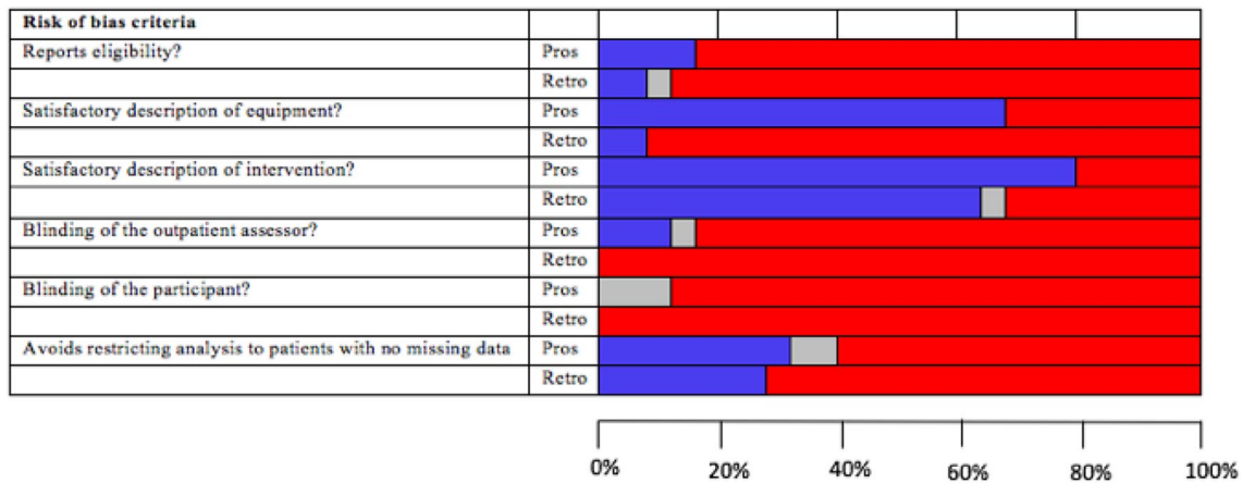
Fig. 2 Graph of risk of bias item for prospective and retrospective studies (blue—studies reporting the criteria, grey—unclear, red—studies omitting the criteria)
