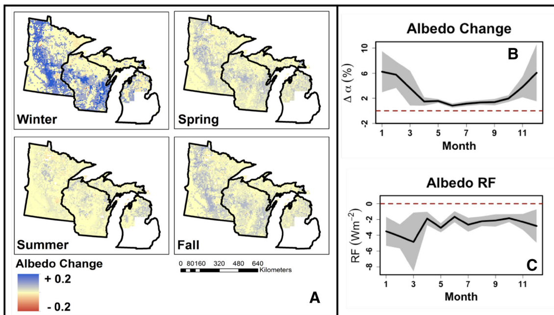
Figure 3. Regional changes in albedo since Euro-American settlement from MODIS-based reconstructions. Panel A shows maps of albedo change for winter (December–February), spring (March–May), summer (June–August), and fall (September–November). Positive values (blue) indicate areas where modern albedo is higher than historic albedo. Panel B shows seasonal variations of albedo change. Panel C shows seasonal variations in the radiative forcing of albedo change adjusted for seasonal insolation. Gray shading on ( B ) and ( C ) indicates a 95% confidence interval.
