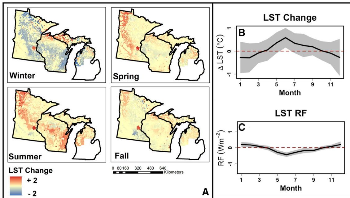
Figure 4. Regional changes in surface temperature since Euro-American settlement from MODIS-based reconstructions. Panel A shows maps of LST changes for winter (December–February), spring (March–May), summer (June–August), and fall (September–November). Negative values (blue) indicate areas where modern surface temperature is lower than historic surface temperature. Panel B shows the seasonal variations of change in surface temperature. Panel C shows seasonal variations in the radiative forcing of surface-temperature change, adjusted for seasonal changes in day length. Gray shading on ( B ) and ( C ) indicates a 95% confidence interval.
