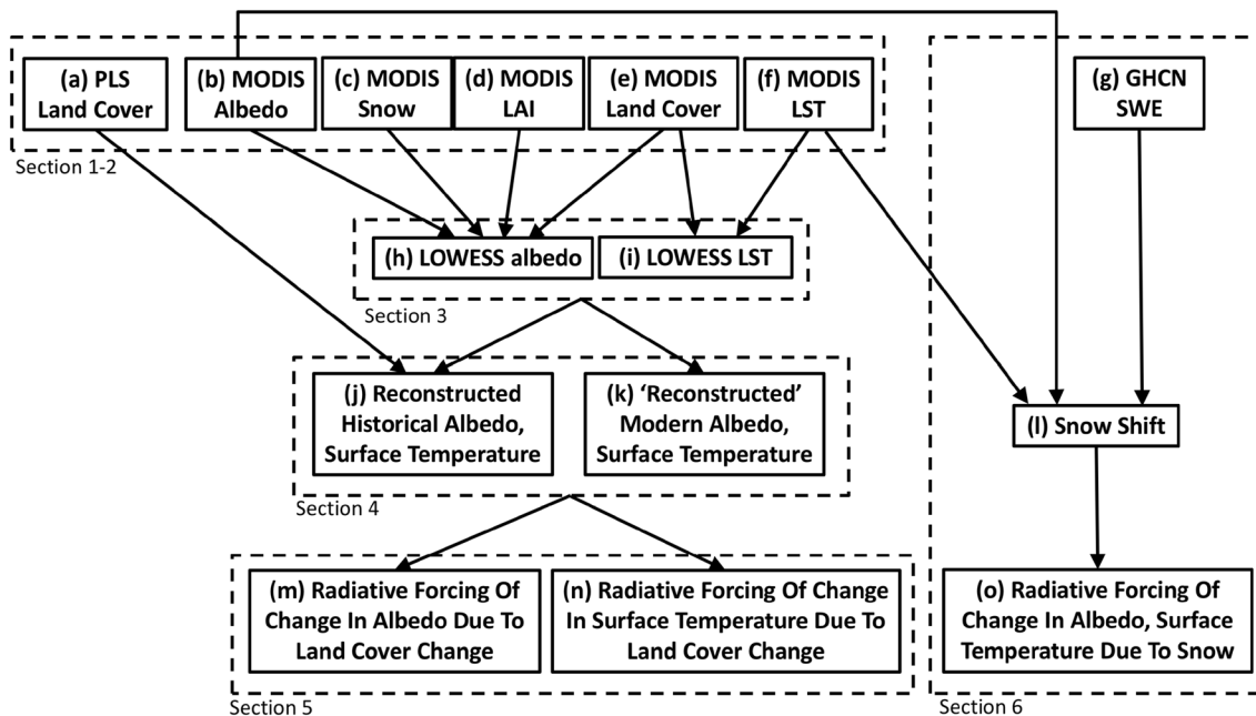
Figure 1. Summary of data (sections 1–2), modeling (section 3), projection (section 4), and calculation (section 5) steps taken to calculate radiative forcings of land-cover change and (section 6) snow change. Section labels refer to italicized methods subheadings.
