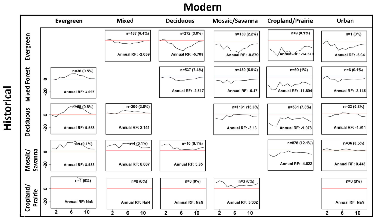
Figure 6. Total vegetation forcing (albedo + LST) for individual vegetation changes.
