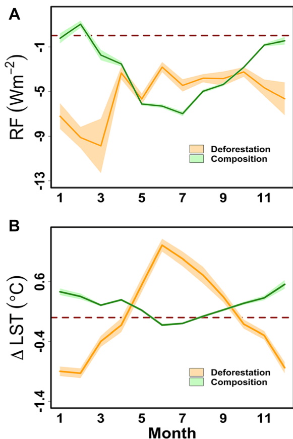
Figure 5. Seasonal patterns of radiative forcing (A) and surface-temperature change (B) for deforestation and composition shift. These two transitions were responsible for 94% of land-cover change.
