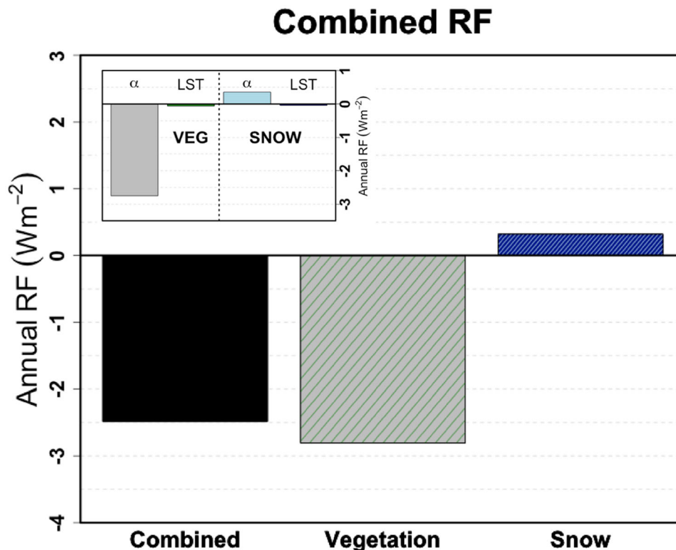
Figure 8. Total radiative forcing of land-use change in the Upper Midwest. Inset shows annual average radiative forcing of each component.
