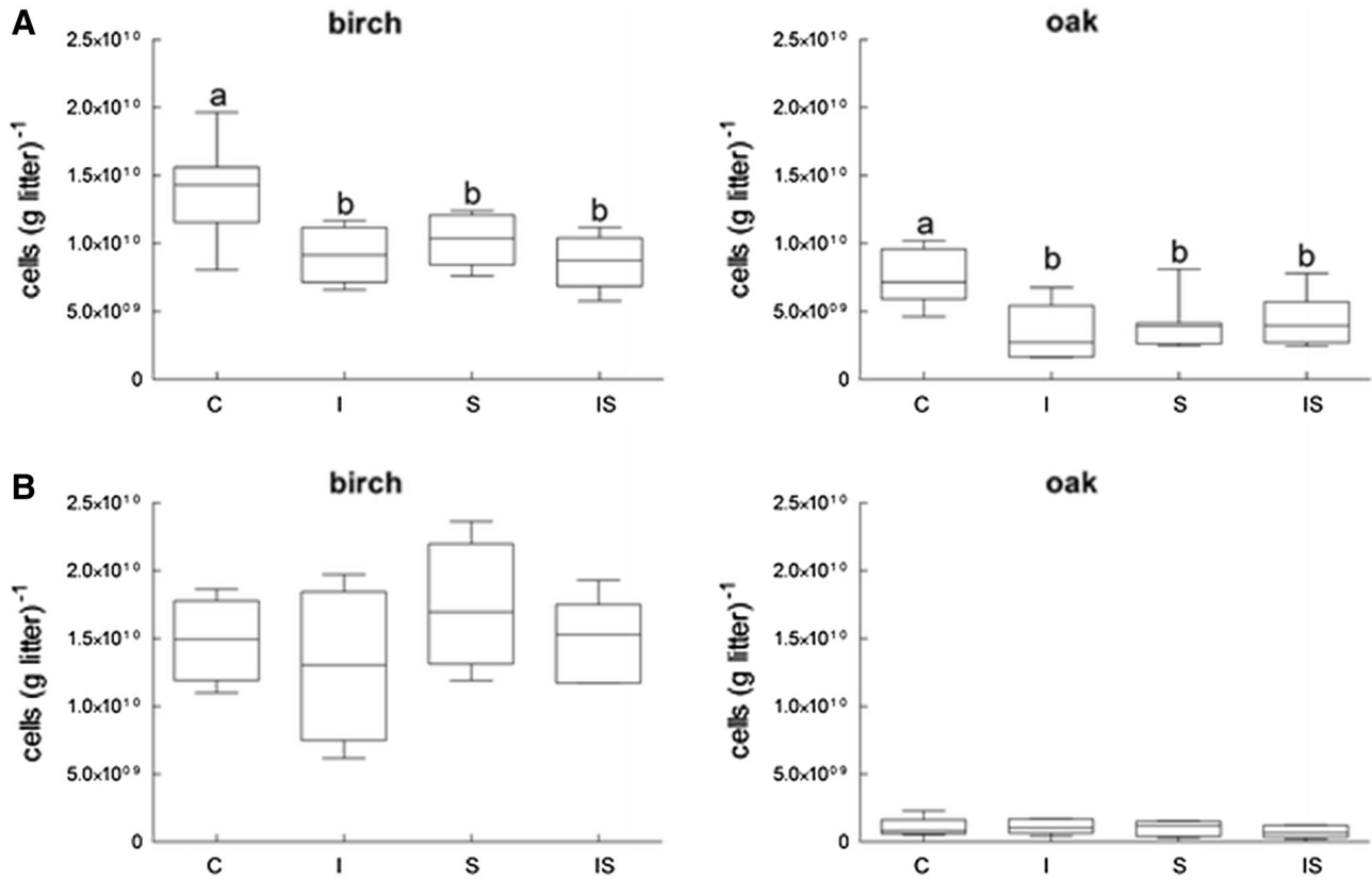
Fig. 4. Bacterial cell densities on birch and oak litter in the aquatic ( A ) and the terrestrial ( B ) environments after 112 days in detritivore-free controls (C) and when isopods (I), snails (S) or isopods and snails (IS) were present. Whisker-box-plots indicate minimum, first quartile, median, third quartile, and maximum ( N = 7 ); different lower-case letters indicate statistically significant differences ( \alpha = 0.05 )
