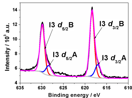
Fig. 5 High-resolution XPS spectra recorded at the iodine region for I-TiO 2 sample. The doping conditions are as follows: reaction voltage of 1.5 V, reaction time of 15 min, and electrolyte concentration of 0.1 M
