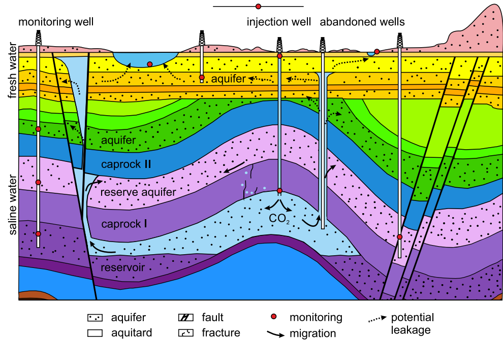
Fig. 4 Schematic illustration of potential leakage pathways associated with geological CO 2 storage
