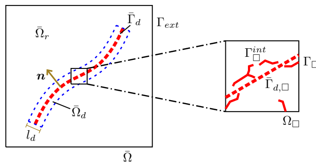
Fig. 2 Macroscopic domain \bar{\Omega} divided into a part \bar{\Omega}_d containing an effective macroscopic discontinuity surface \bar{\Gamma}_d , and a part \bar{\Omega}_r that is free from macroscopic discontinuities. The width l_d of the discontinuity region \bar{\Omega}_d is also shown
