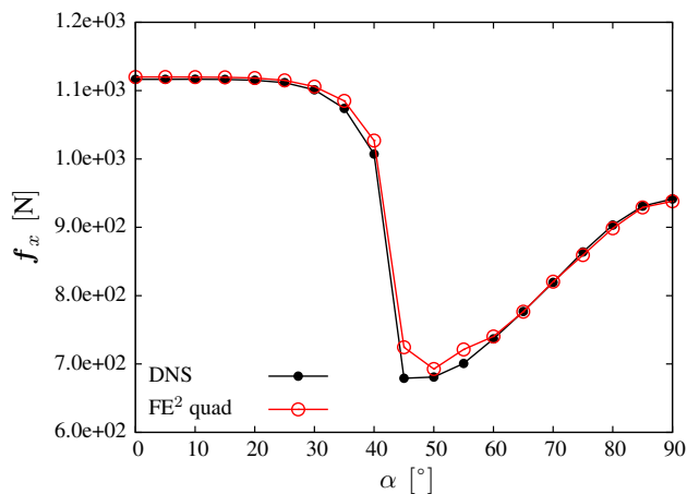
Fig. 13 Plate with soft band considered in Example 4.3. Horizontal reaction force versus angle of the soft band computed with DNS and FE 2
