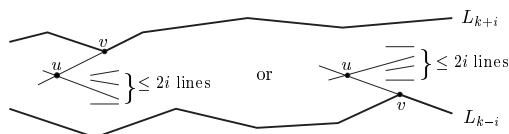
Fig. 1. The charging argument for Lemma 2.1.
