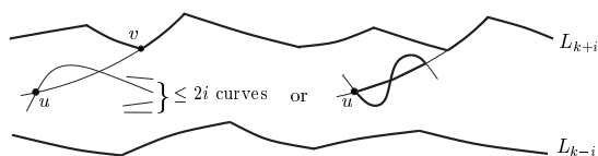
Fig. 2. The charging argument for Lemma 3.1, with s = 2 . (In the scenario to the left, u is charged to a vertex v \in L_{k+i} \setminus L_{k+i+1} . In the scenario to the right, u is charged to a 2-lens in \Lambda_i^{(s)} , shown in bold.)
