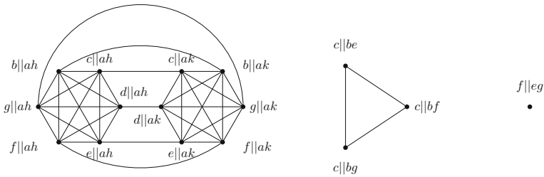
Fig. 5 The graph \mathcal{C}(\delta_{\mathcal{N}_1}) , where \mathcal{N}_1 is the labelled level-1 network depicted in Fig. 1
