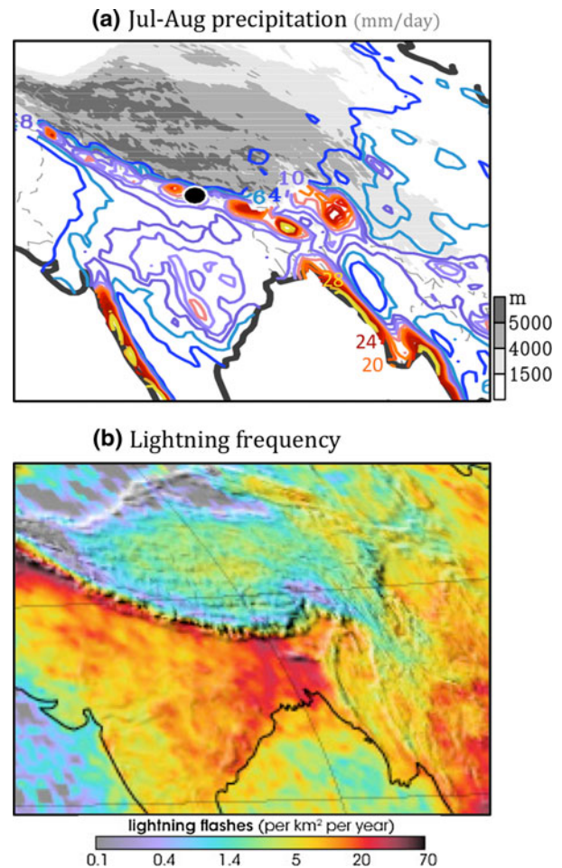
Fig. 1 a July–August climatology of precipitation ( contours ; mm/day) and the topography ( shadings ), and b annual lightning frequency between 1997 and 2002 derived from the Lightning Imaging Sensor onboard the TRMM satellite and between 1995 and 2000 by the Optical Transient Detector ( Source : NASA Earth Observatory Webpage). The black dot in a marks Kathmandu, Nepal's capital city
