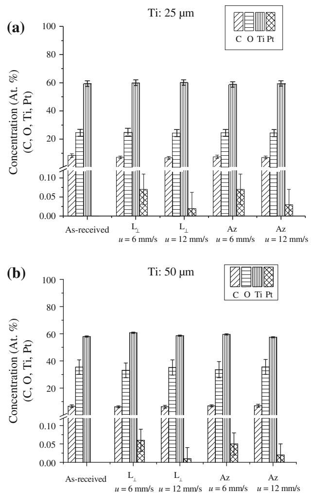
Fig. 8 Concentrations of different elements in laser-treated, a 25 μm-thick and b 50 μm-thick Ti samples
