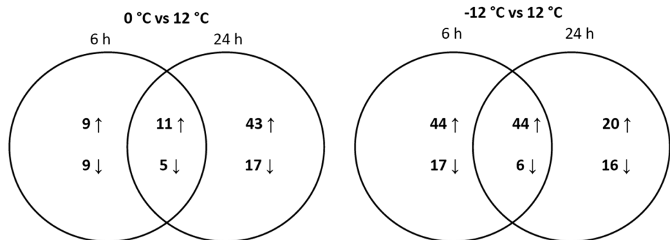
Fig. 1 The distribution of differentially expressed genes in Glaciozyma antarctica PI12 at 0 °C and – 12 °C
